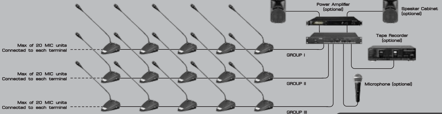
SYSTEM CONNECTION DIAGRAM
